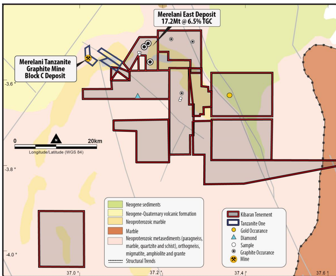
Figure 1 Geological plan showing Mineral Resource estimate and interpretation
