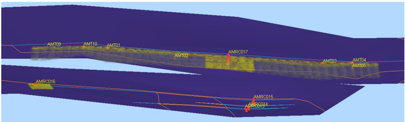
Figure 6 3D View of Southern Zone block model showing drill holes and trenches (red), geological mapping strings, topographic DTM and resource blocks coloured on resource classification (yellow = Inferred, grey = unclassified). View looking up towards south. Strike length of modelled mineralisation is 2,300 m.
