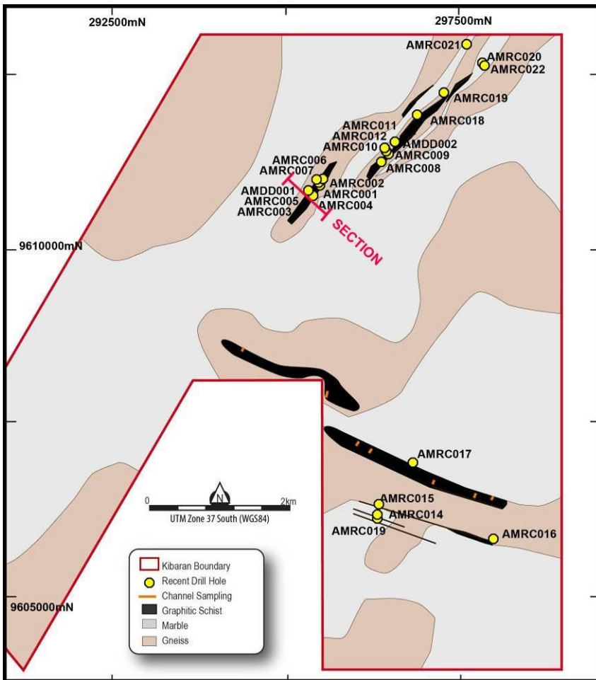
Figure 2 Location of drilling at Merelani East deposit
