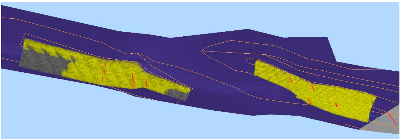
Figure 5 3D View of Northern Zone block model showing drill holes (red), geological mapping strings, topographic DTM and resource blocks coloured on resource classification (yellow = Inferred, grey = unclassified). View looking up towards west-north-west. Strike length of Inferred Mineral Resource approximately 1,800 m.
