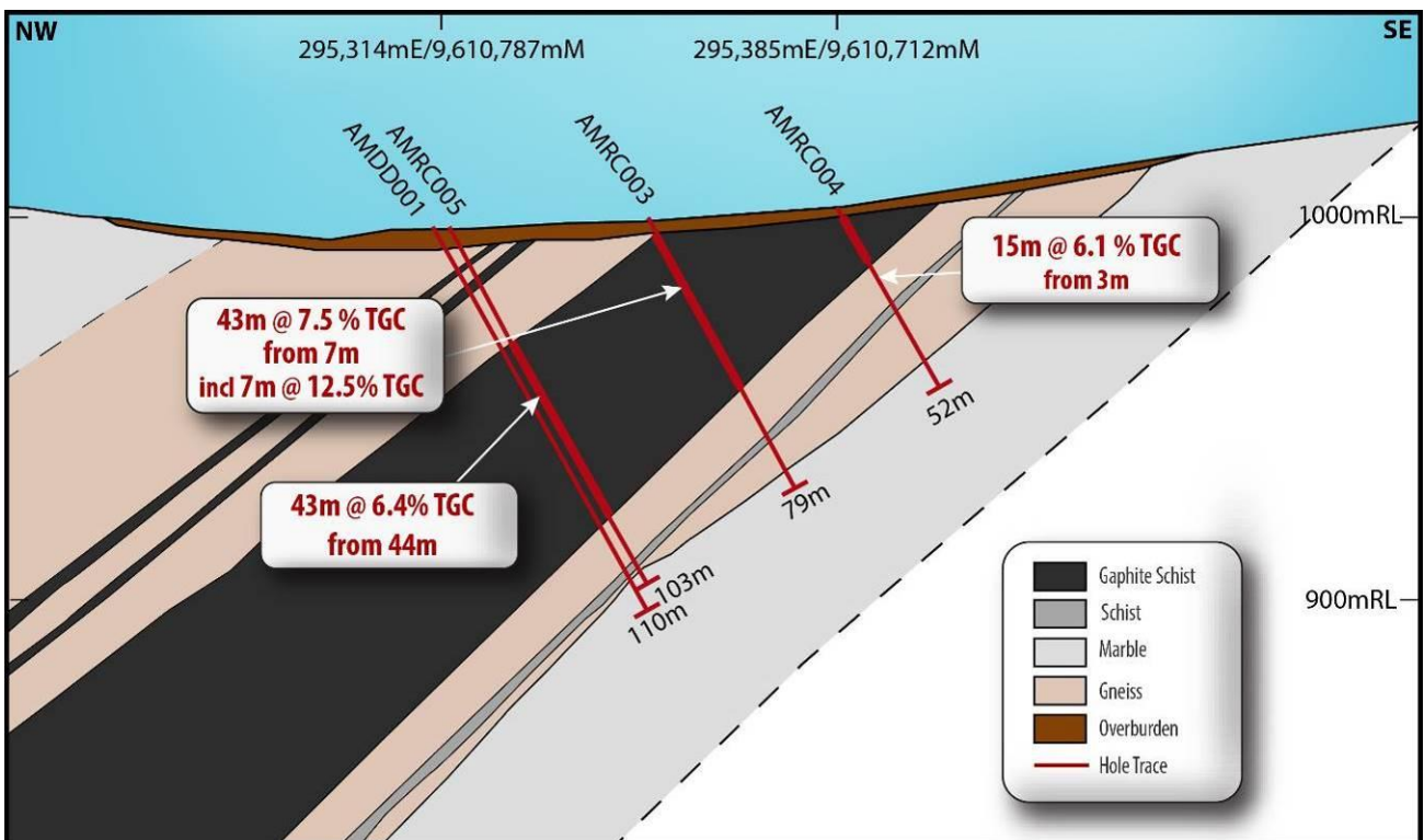
Figure 3 Geological cross-section of Merelani East deposit
